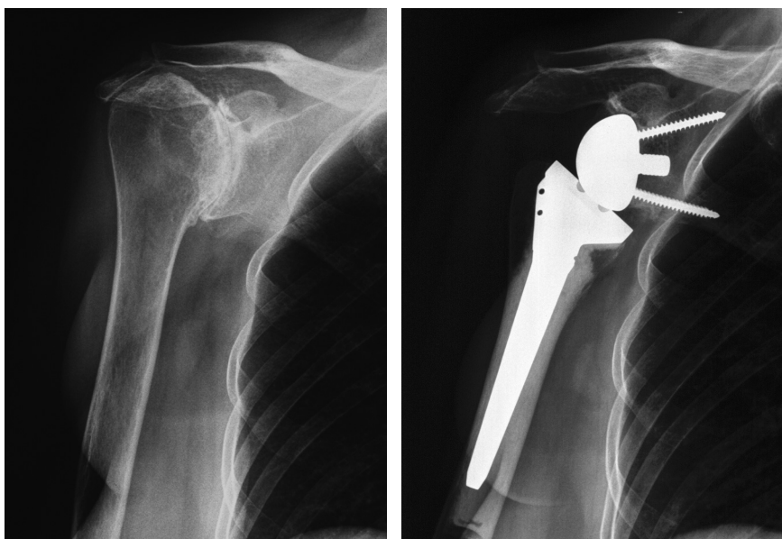
Figure 1. Delta III prosthesis in CTA type V according to Hamada.
